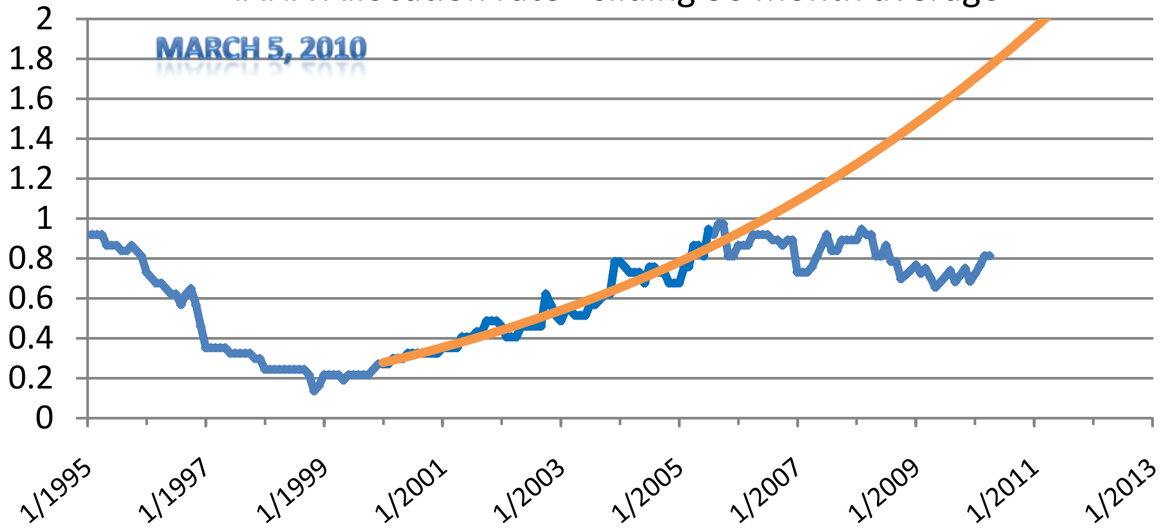
IANA Allocation rate - sliding 36 month average
